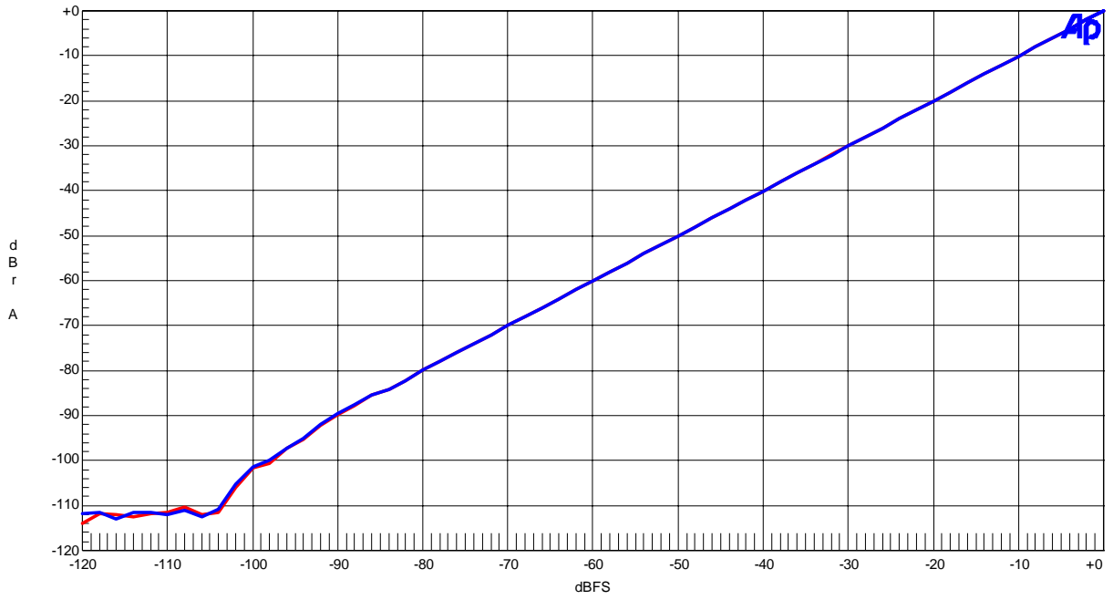
Figure1-7.Linearity (fin=1kHz)
