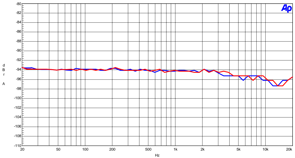
Figure1-6. THD+N vs. Input Frequency (Input level=0dBFS)
