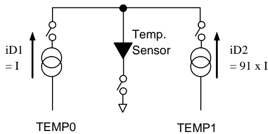
Figure 5 Temperature Measurement
