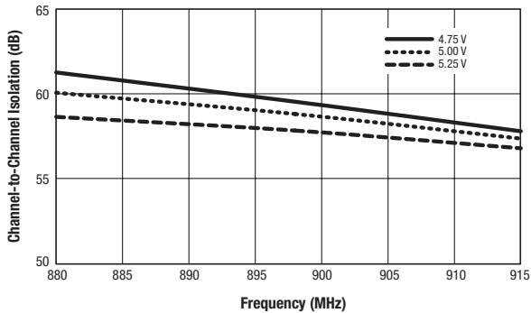
Figure 27. Channel A To Channel B Isolation vs Frequency and Supply Voltage
