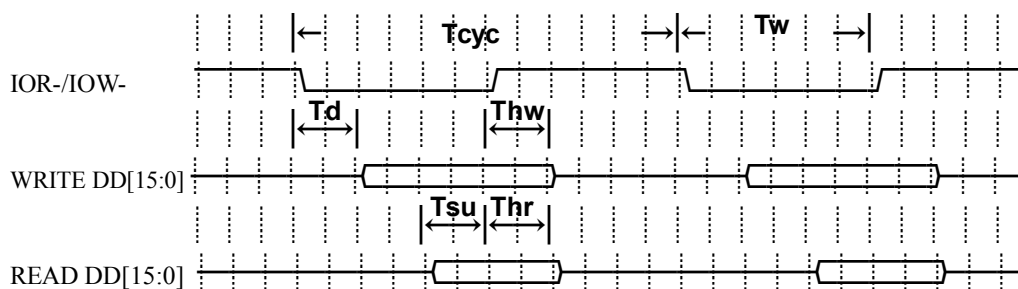
Figure 6.7 - Timing Diagram of CompactFlash
