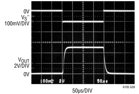
Step Response V_{SENSE} = 0\text{V to } 100\text{mV}, C_L = 1000\text{pF}, V_{S^+} = 0\text{V}
