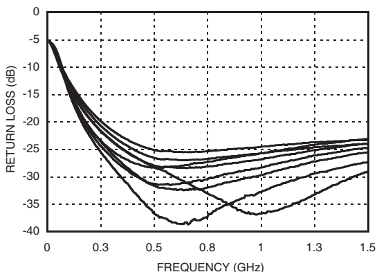
Input Return Loss [2] (Only Major States are Shown)
