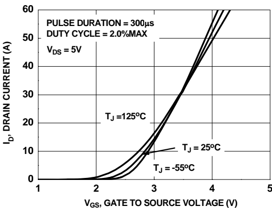
Figure 16. Transfer Characteristics
