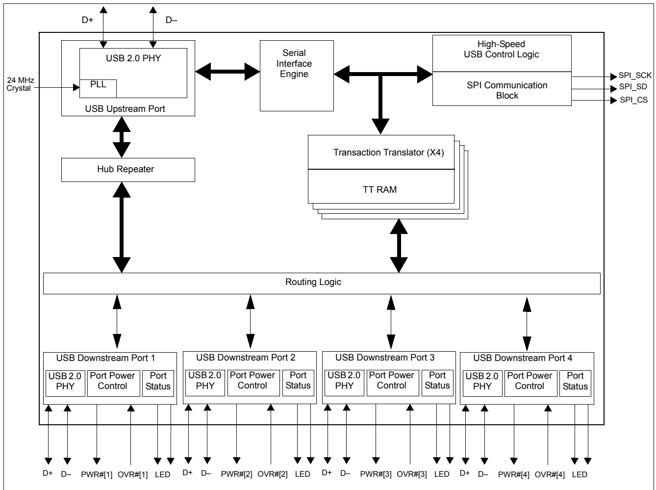
Figure 1-1. Block Diagram
