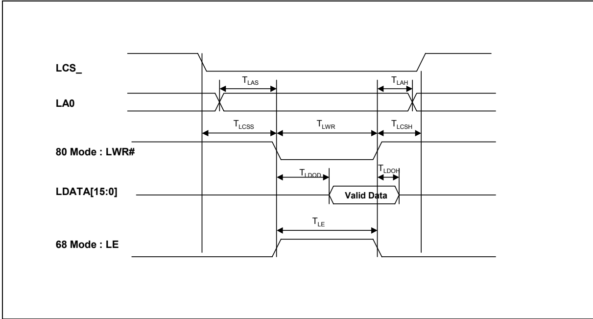
Figure 5.4 LCD Interface Timing Diagram
