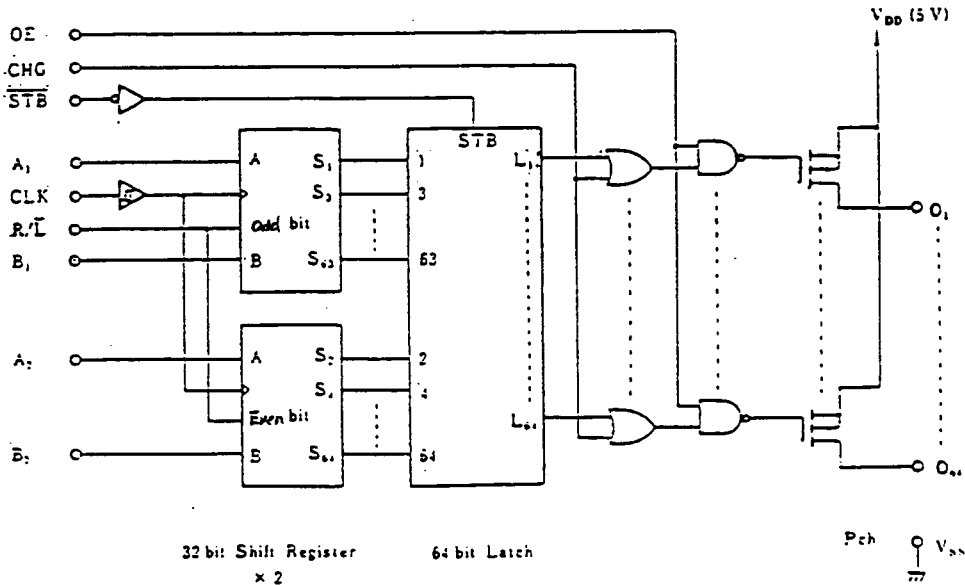
(BLOCK DIAGRAM)
