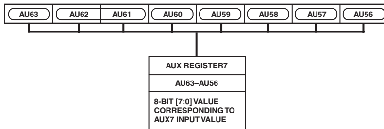
Figure 38. AUX Register 7
