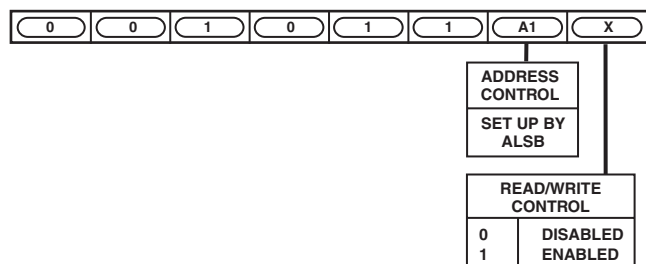
Figure 4. Slave Address
