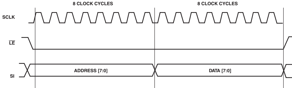
Figure 10. SPI Timing Mode 1
