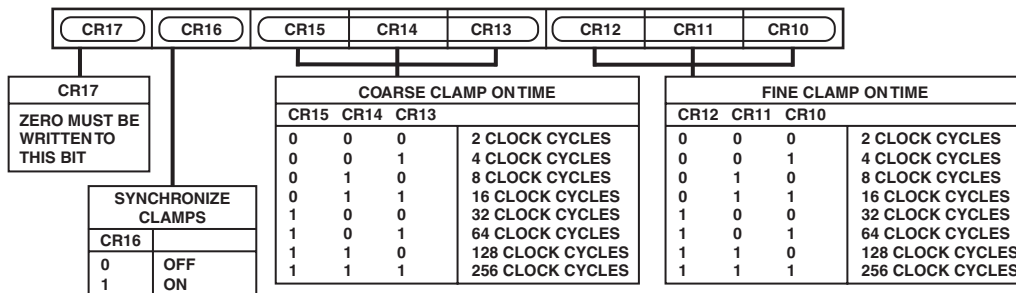
Figure 26. Clamp Register 1
