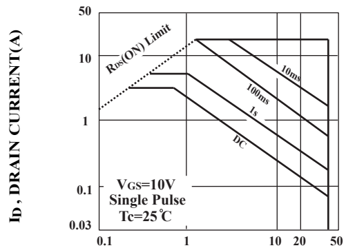
FIG.10 Maximum Safe Operating Area
