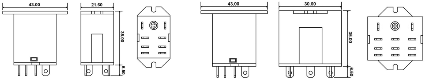
1 & 2 POLE WITH FLANGE
