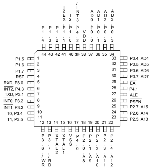
44-Pin QFP
