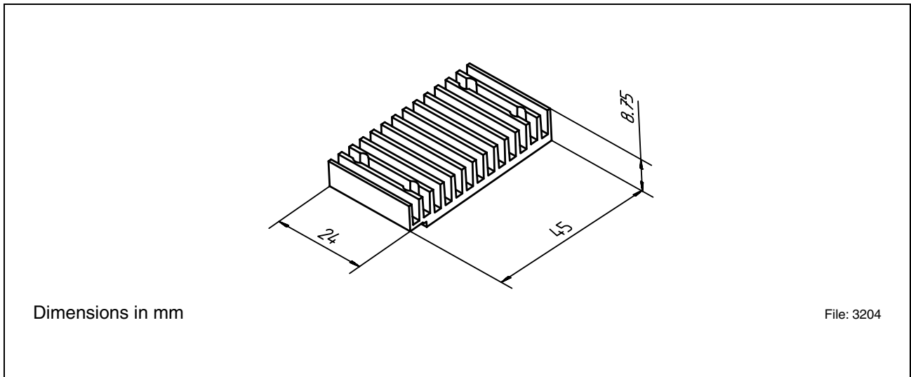
Figure 1 Heatsink PAROLI Backplane Module
