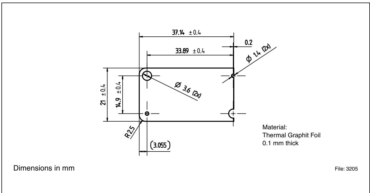
Figure 2 Heat Dissipation Foil
