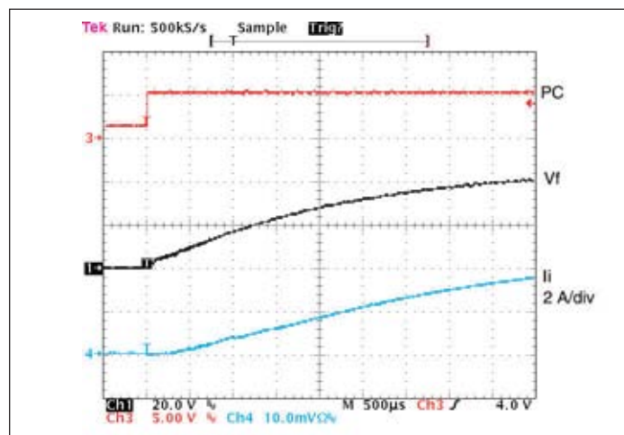
Figure 3 — Vf turn-on waveform with inrush current – PC enabled at full load, 48 Vin
