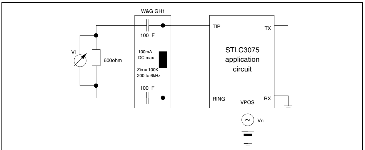
Figure 17. PSRRC Power supply rejection Vpos to 2W port PSSRC = 20\text{Log}|V_n/V_{II}|
