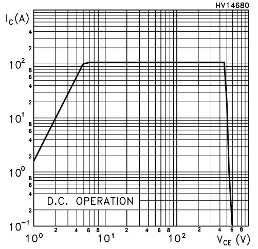
Figure 16: Turn-Off SOA
