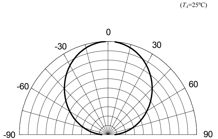
Radiation Diagram
