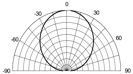
◎ Radiation Diagram
