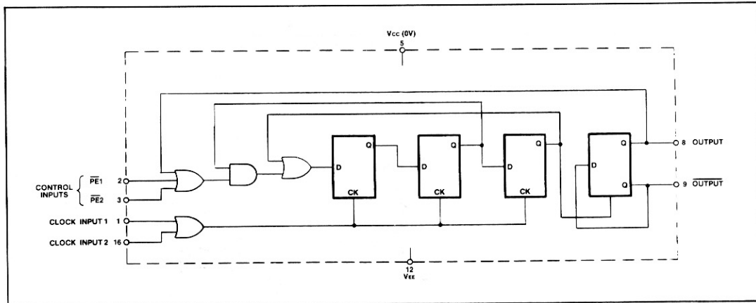
Fig.2 Functional diagram
