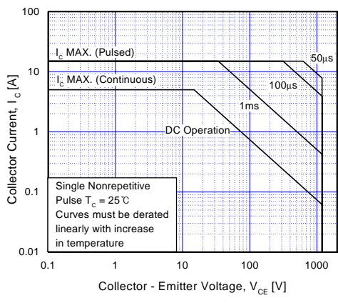
Fig 15. SOA Characteristics
