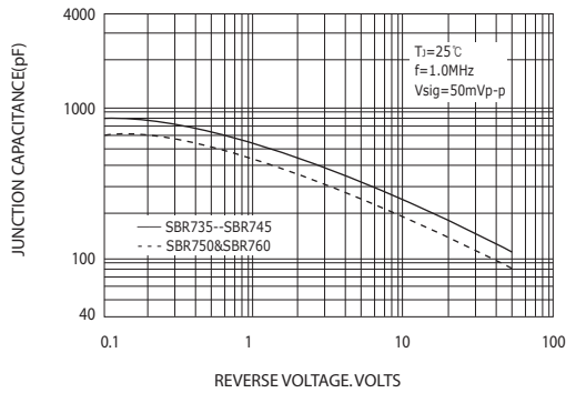
FIG.5-TYPICAL JUNCTION CAPACITANCE
