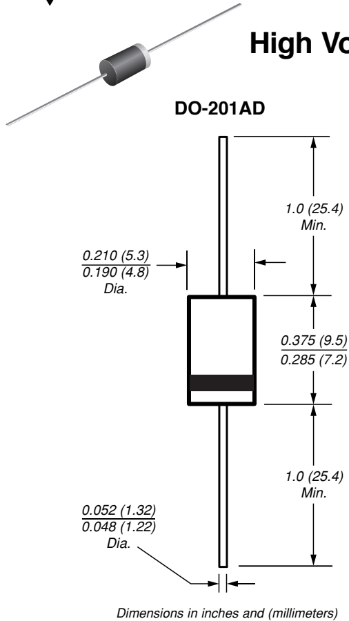
Dimensions in inches and (millimeters)
