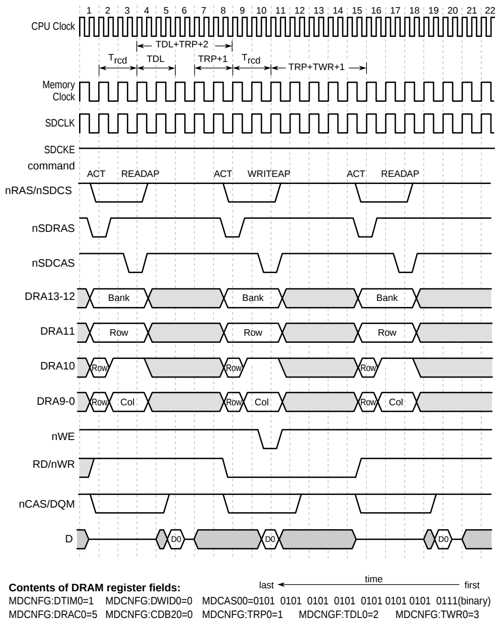
Figure 10-8. SDRAM 1-Beat Read/Write/Read Timing for 4 Bank x 4 M x 4 Bit Organization (64 Mbit)
