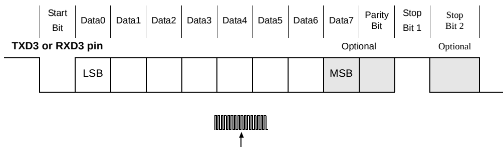
Figure 11-28. Example UART Data Frame
