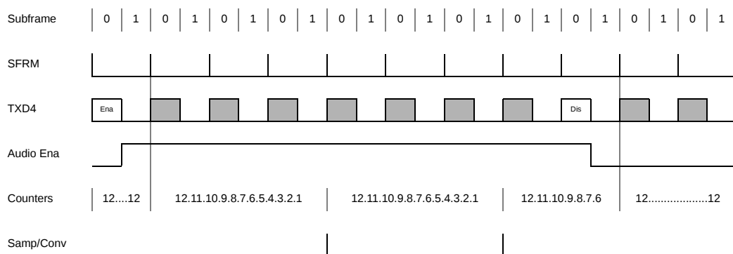
Figure 11-31. MPC/Codec Sampling Counter Synchronization
