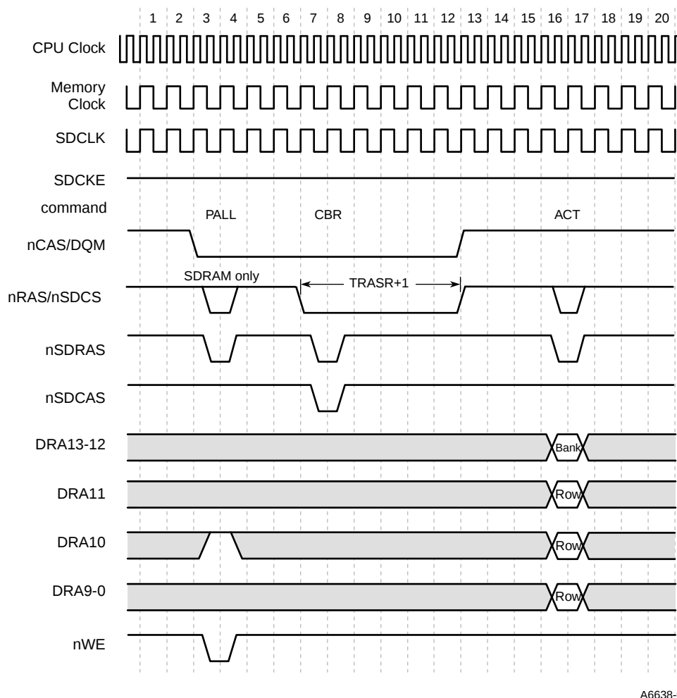
Figure 10-11. DRAM/SDRAM CBR Refresh Cycle
