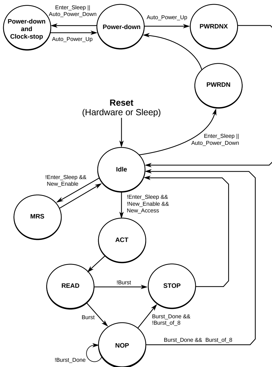
Figure 10-19. SMROM State Machine
