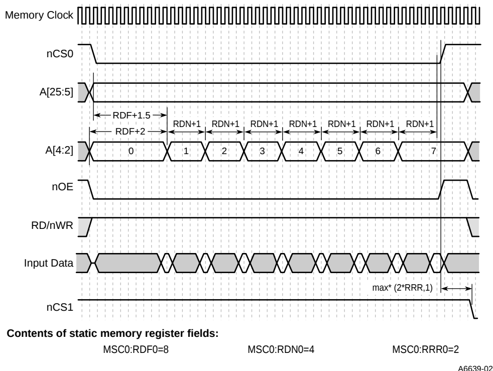
Figure 10-12. Burst-of-Eight ROM or Flash Read Timing Diagram
