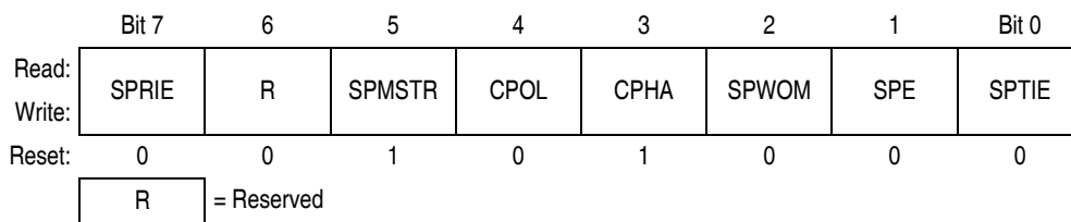
Figure 15-13. SPI Control Register (SPCR)
