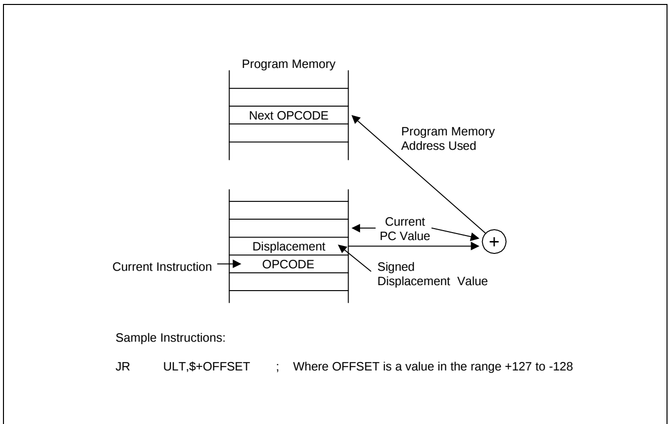
Figure 3-13. Relative Addressing
