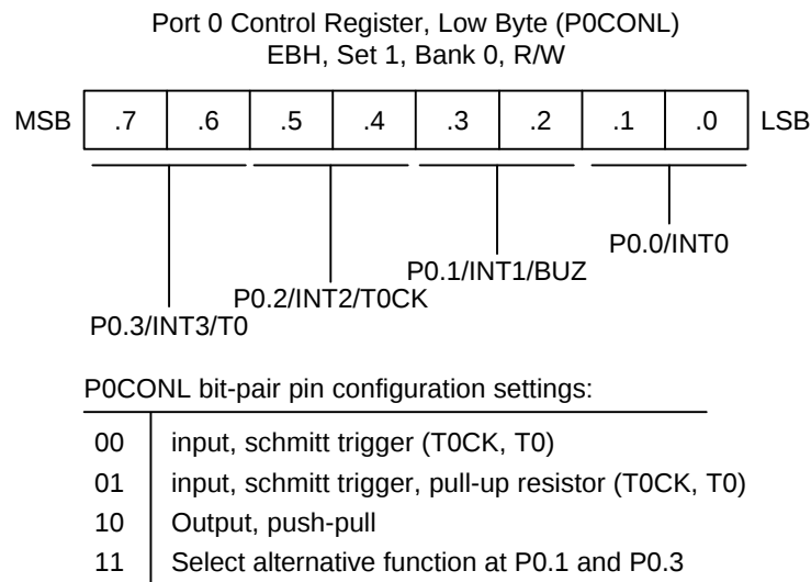
Figure 9-3. Port 0 Control Register (P0CONL)
