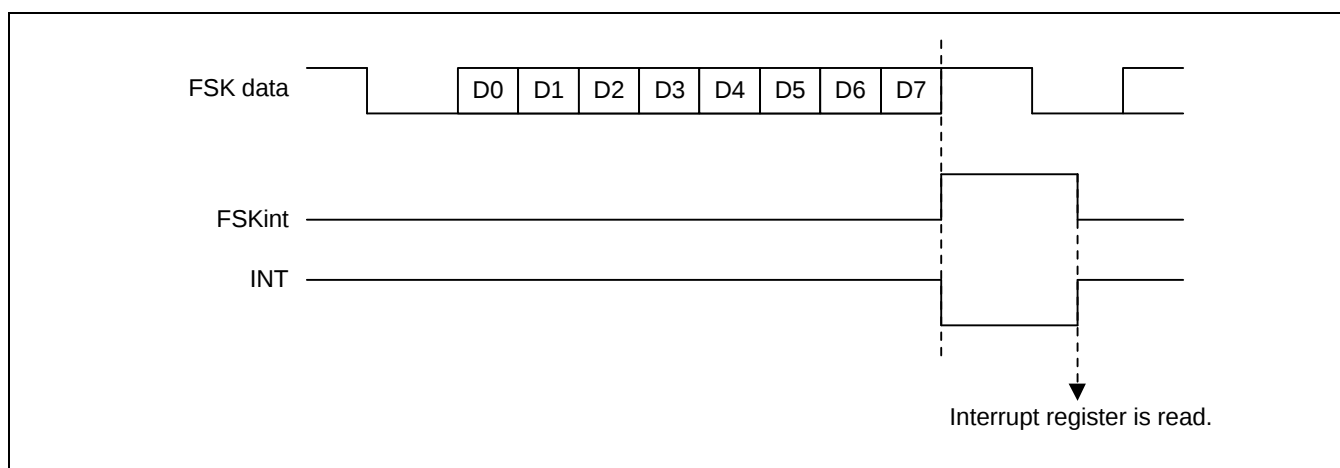
Figure 14-5. Sequence to Receive an FSK Data Byte
