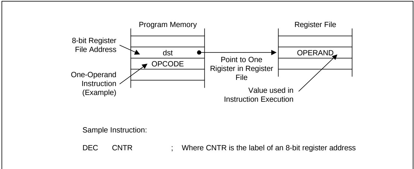
Figure 3-1. Register Addressing
