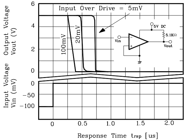
Fig. 6 V_{IN}, V_{OUT}-t_{rsp}
