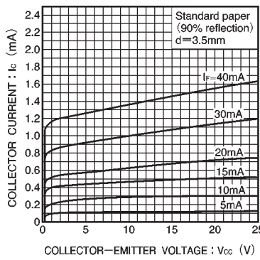
Fig.5 Output characteristics
