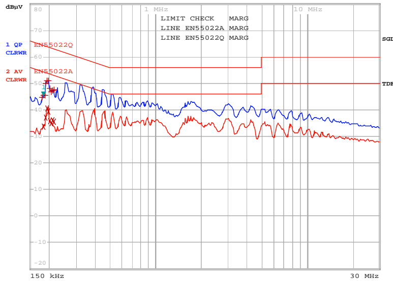
Figure 19 – Conducted EMI at 230 VAC.
