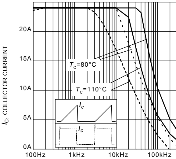
Figure 1. Collector current as a function of switching frequency ( T_j \leq 150^\circ\text{C} , D = 0.5 , V_{CE} = 600\text{V} , V_{GE} = 0/+15\text{V} , R_G = 81\Omega )
