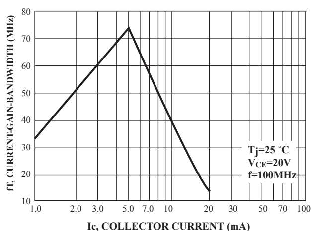
Figure .2 Current-Gain-Bandwidth
