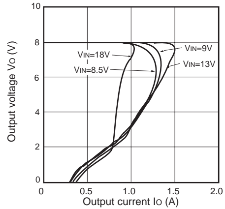
Fig.6 Overcurrent Protection Characteristics (PQ080RDA1SZH)
