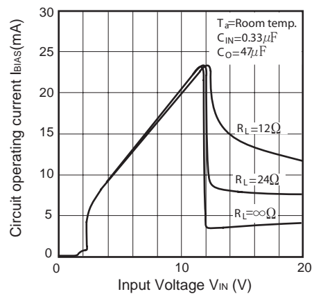
Fig.18 Circuit Operating Current vs. Input Voltage (PQ120RDA1SZH)
