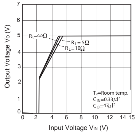
Fig.10 Output Voltage vs. Input Voltage (PQ050RDA1SZH)
