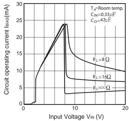
Fig.16 Circuit Operating Current vs. Input Voltage (PQ080RDA1SZH)
