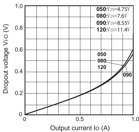
Fig.19 Dropout Voltage vs. Output Current (PQxxxRDA1SZH)
