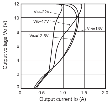
Fig.8 Overcurrent Protection Characteristics (PQ120RDA1SZH)
