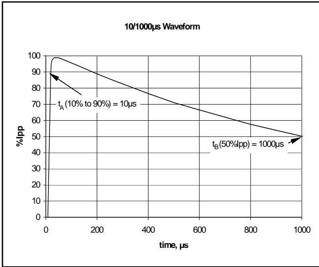
Surge Current Pulse Waveform 10/1000μs
