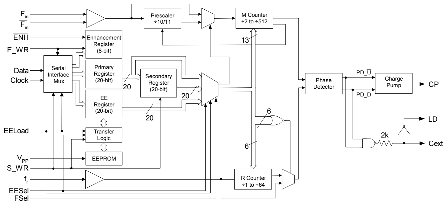
Figure 1. Block Diagram
