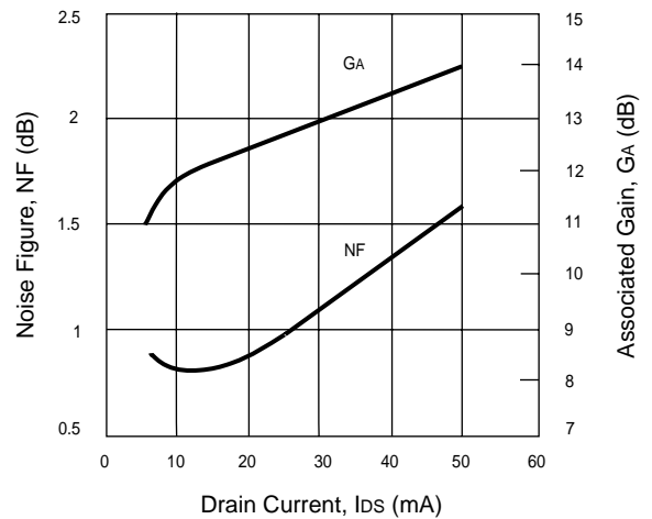
NOISE FIGURE AND ASSOCIATED GAIN vs. DRAIN CURRENT V DS = 3 V, f = 4 GHz
