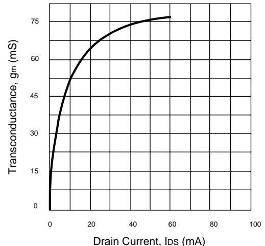
TRANSCONDUCTANCE vs. DRAIN CURRENT V DS = 3 V
