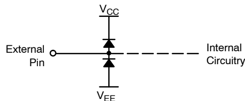
Figure 23. Internal ESD Protection
