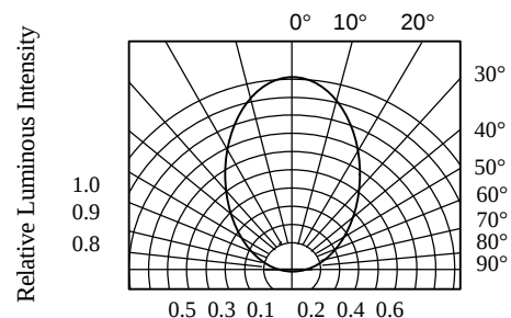
FIG.6 RADIATION DIAGRAM
