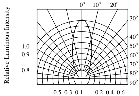
FIG.6 RADIATION DIAGRAM
