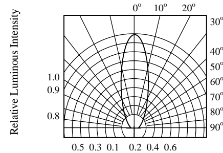
FIG.6 RADIATION DIAGRAM
