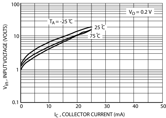
FIG.16 Input Voltage versus Output Current
