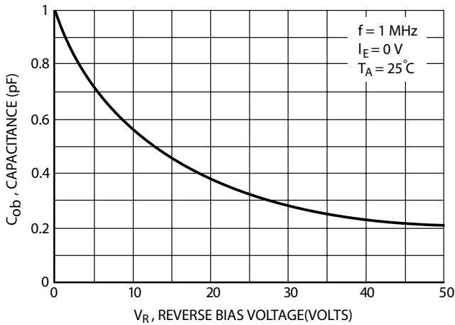
FIG.14 Output Capacitance
