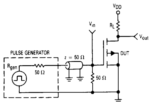
Figure 14. Switching Test Circuit
