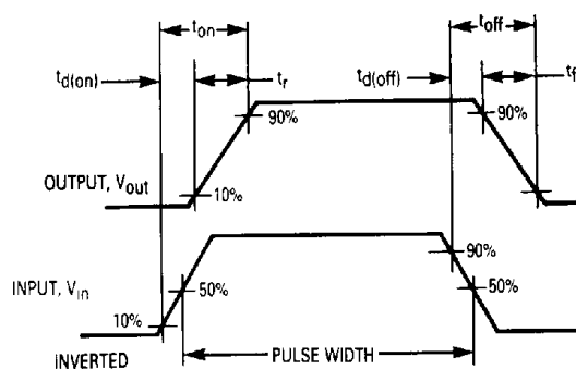
Figure 15. Switching Waveforms
