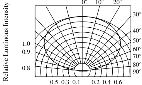
FIG.6 RADIATION DIAGRAM
