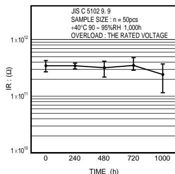
Fig.22 Insulation resistance
