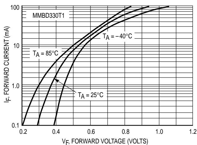
Figure 9. Forward Voltage
