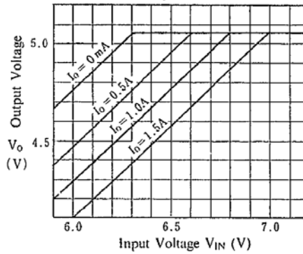
ML7812 Dropout Characteristics
