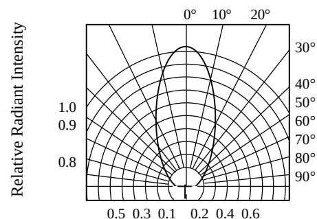
FIG.5 RADIATION DIAGRAM
