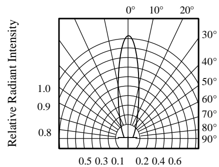
FIG.5 RADIATION DIAGRAM
