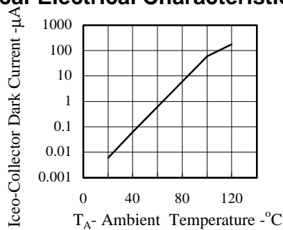
FIG.1 COLLECTOR DARK CURRENT VS AMBIENT TEMPERATURE
