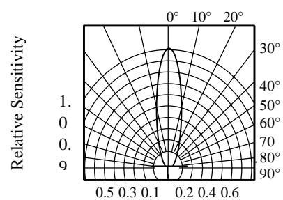
FIG.6 SENSITIVITY DIAGRAM
