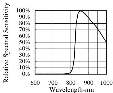
FIG.5 RELATIVE SPECTRAL SENSITIVITY VS. WAVELENGTH
