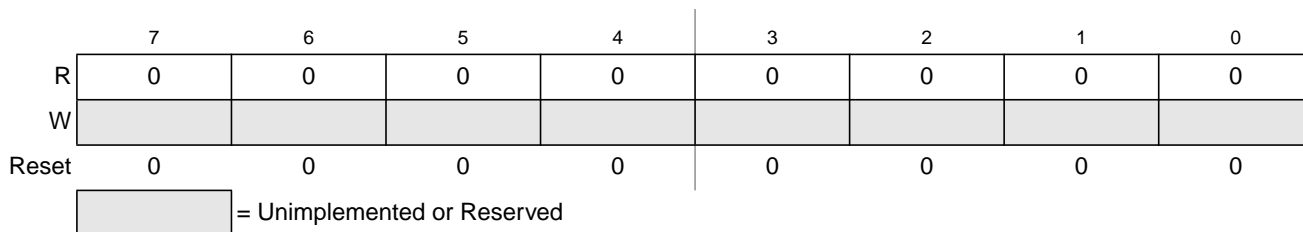
Figure 28-22. RESERVED3
